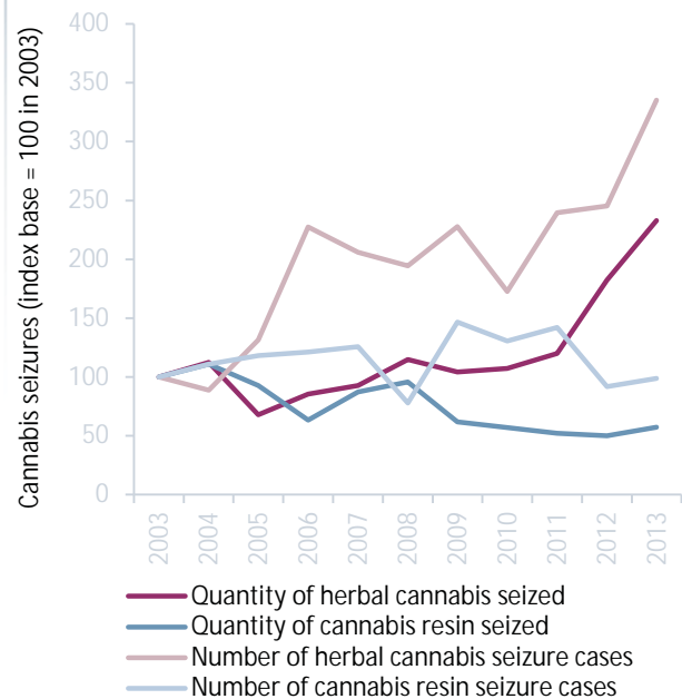
FIG. 66. Number and quantity of cannabis seizures in Europe, 2003-2013
