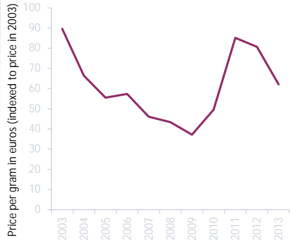
FIG. 49. Purity-adjusted price per gram of heroin the United Kingdom, 2003-2013
